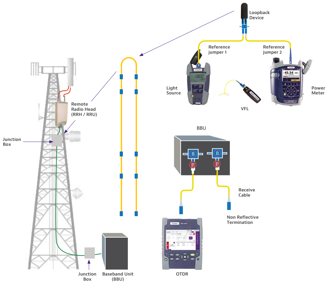
Figure 1. FTTA Fiber Testing
