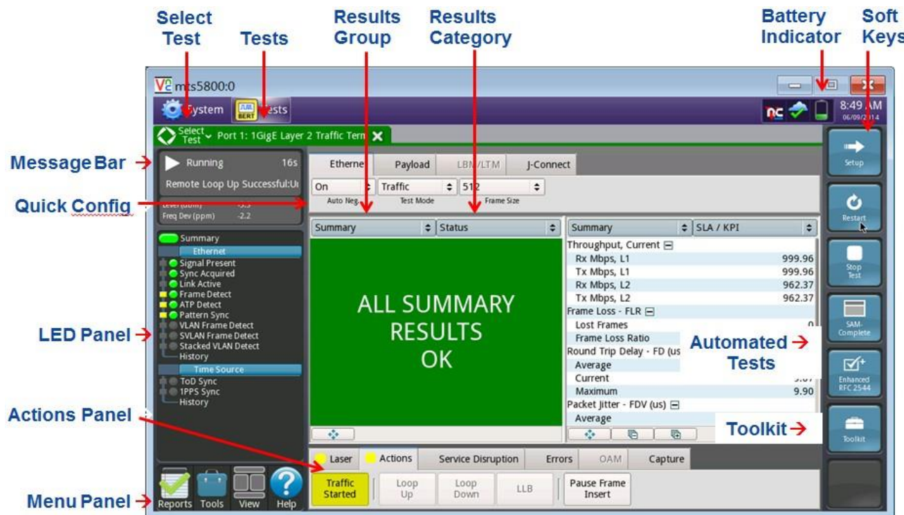
Figure 6: MTS Tests User Interface
