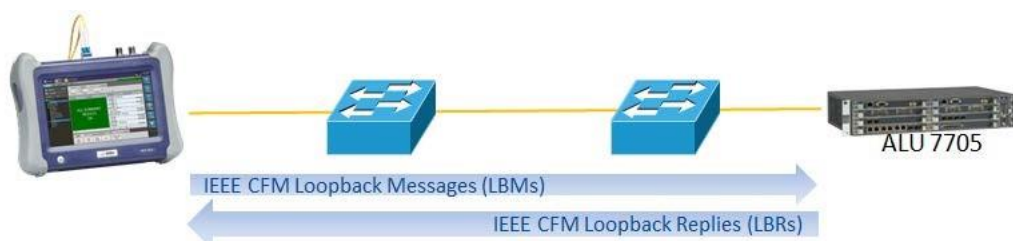
Figure 2: MTS to ALU 7705
