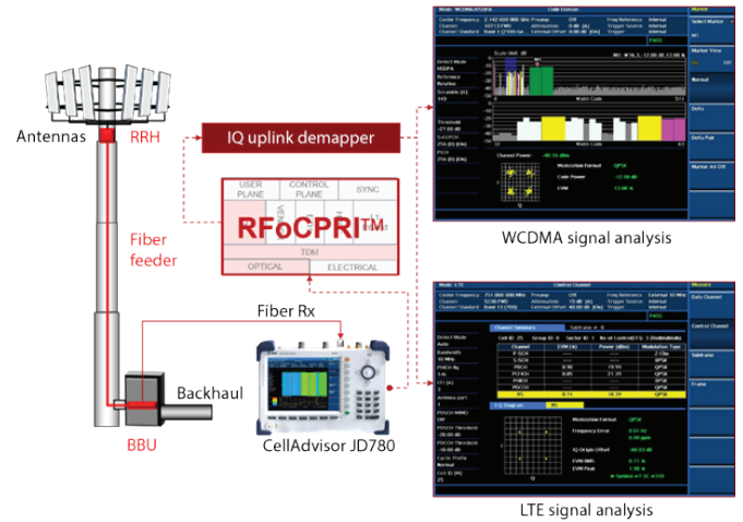
Signal analysis via CPRI
