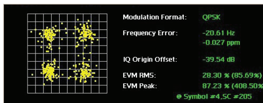
Reference Signal EVM at DAS
