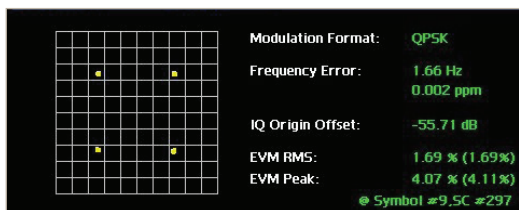
Reference Signal EVM at eNodeB
