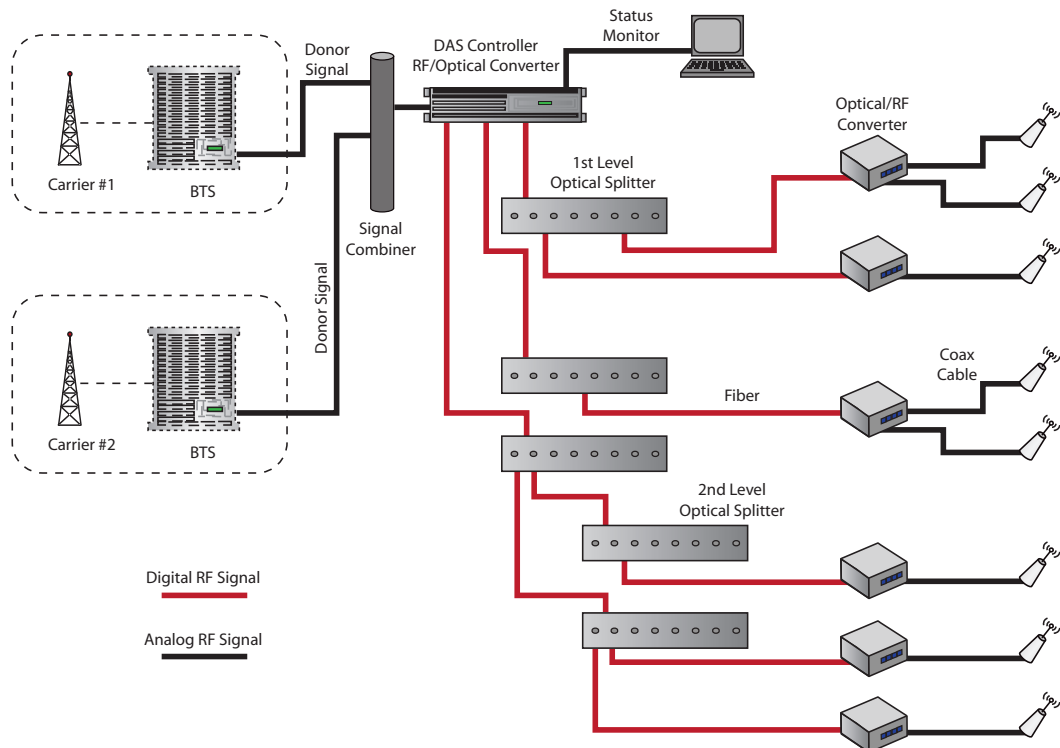
Distributed Antenna System (Hermes Wireless Solutions)
