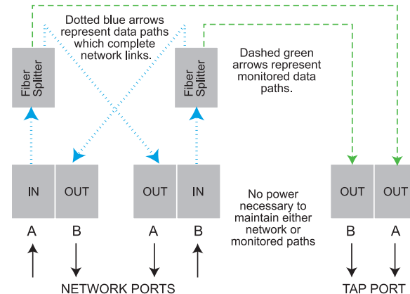
Figure 3: Passive Optical TAP
