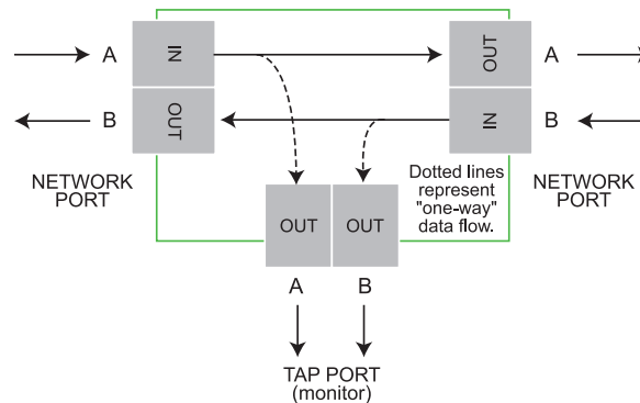
Figure 1: General TAP Functional Diagram
