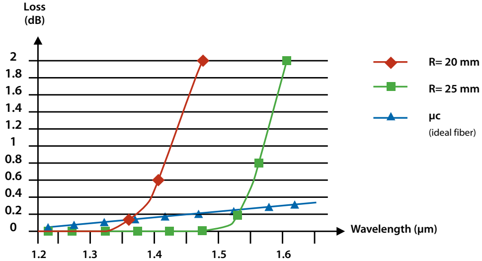
Figure 1: R Radius of curvature of fiber
