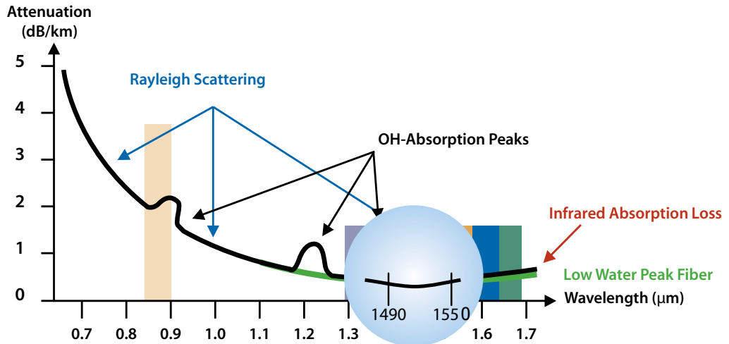
Figure 2: Fiber attenuation as a function of wavelength
