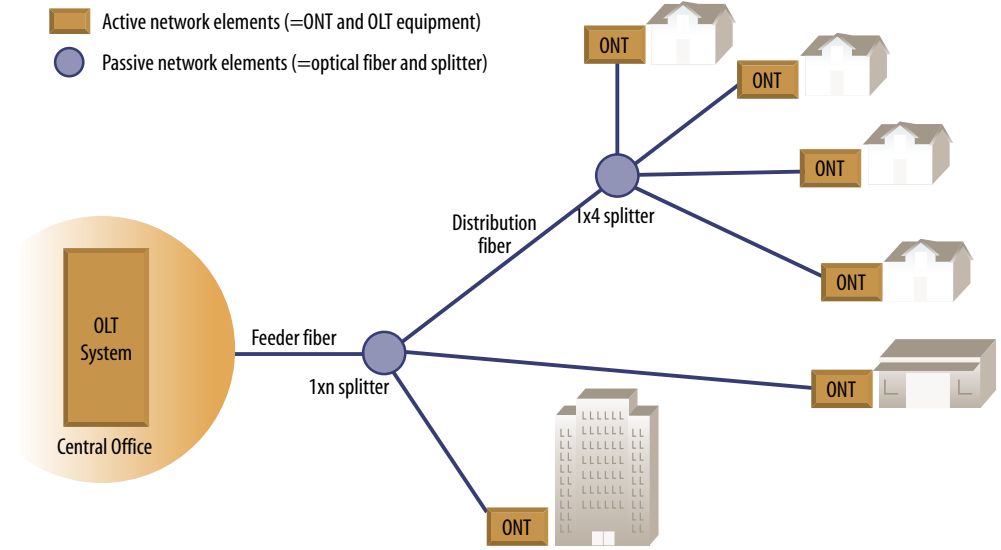
Figure 3: Active and passive network elements
