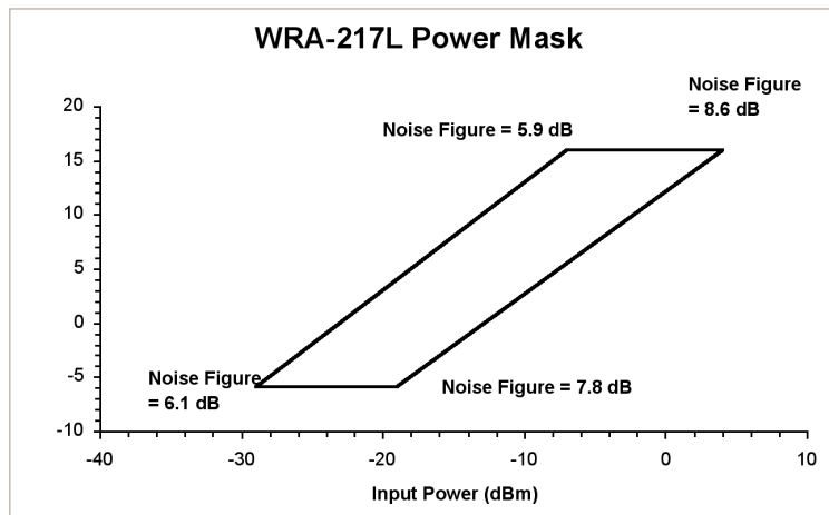
Figure 1: Power mask with noise figures 2 for WRA-217L
