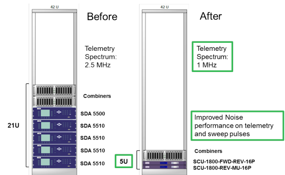
SCU-1800 saves rack space and reduces combining network with 16 ports available for reverse sweep
