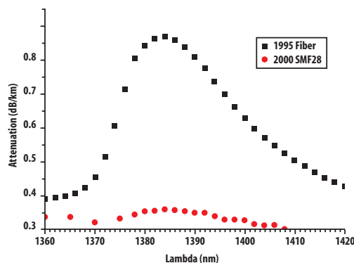
Fiber Attenuation Comparison
