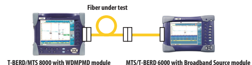
Test setup with T-BERD/MTS 8000 and full band broadband source module
