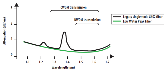
Fiber attenuation as a function of wavelength
