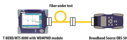
Test setup with T-BERD/MTS 8000 and handheld broadband source
