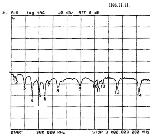
SA7000 plot shows 300kHz - 3GHz
