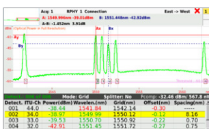
Figure 3. OCC-4056C optical channel verifier screenshot
