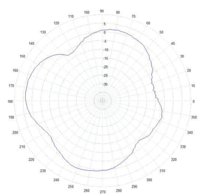
5500 MHz – Azimuth Plot
