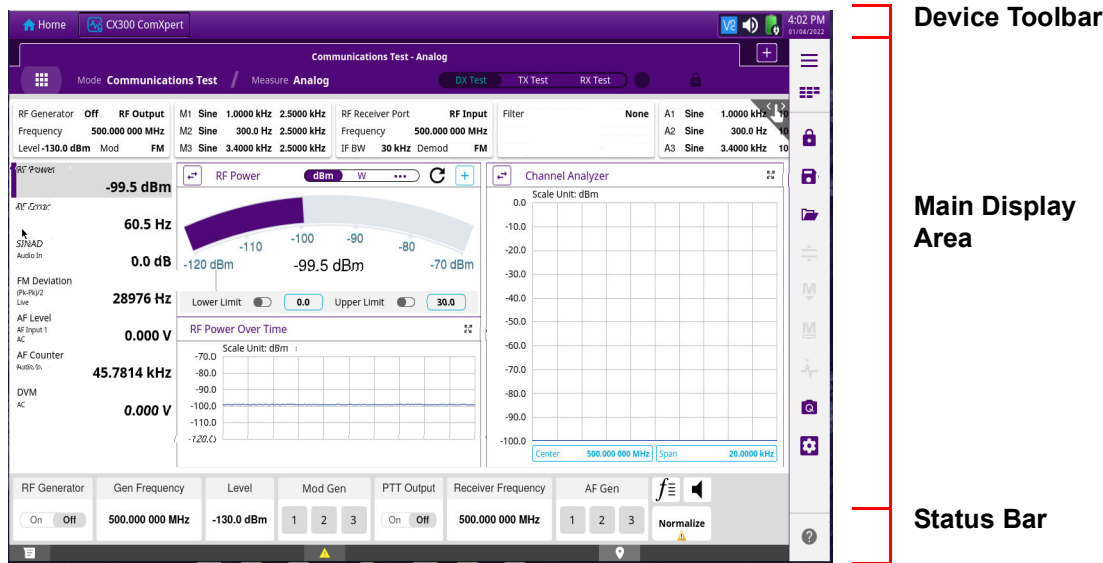
Figure 2-4 CX300 ComXpert Screen Layout
