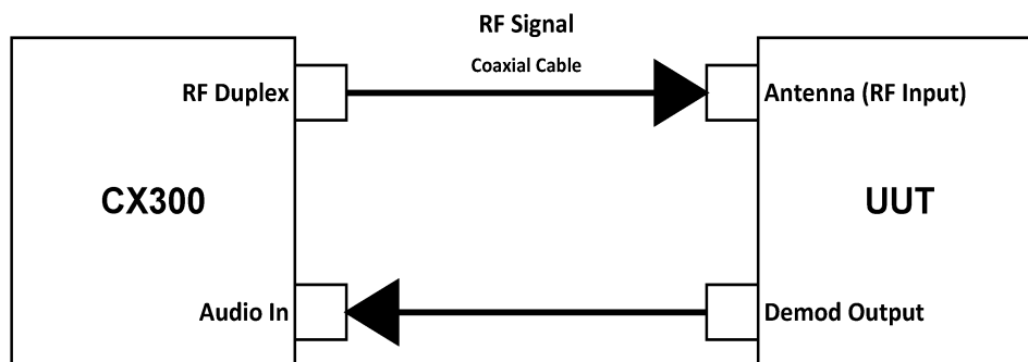
Figure 6-9 Channel Power Measurements Setup Diagram
