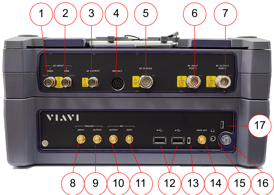
Figure 1-2 CX300 Top Panel Controls and Connectors
