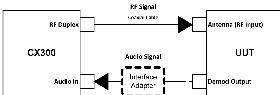
Figure 6-8 Receiver Test Setup Diagram
