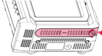
Figure 8-1 Battery Door Cover Thumbscrew
