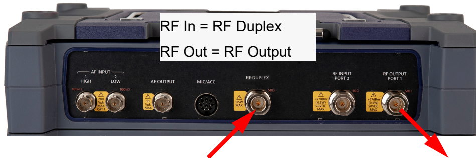
Figure 6-3 RF Output/RF Duplex Two Port Duplex Test Setup
