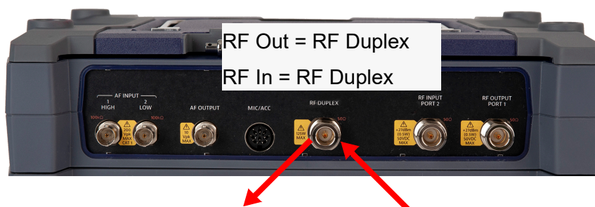
Figure 6-1 One Port Duplex Test Setup
