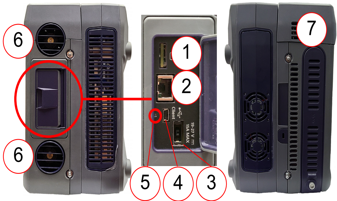
Figure 1-3 CX300 Side Panel Controls and Connectors
