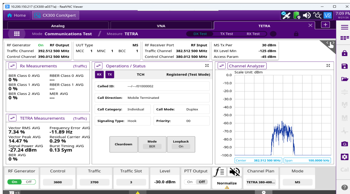
Figure 3-12 TETRA Loopback BER Test Results Screen
