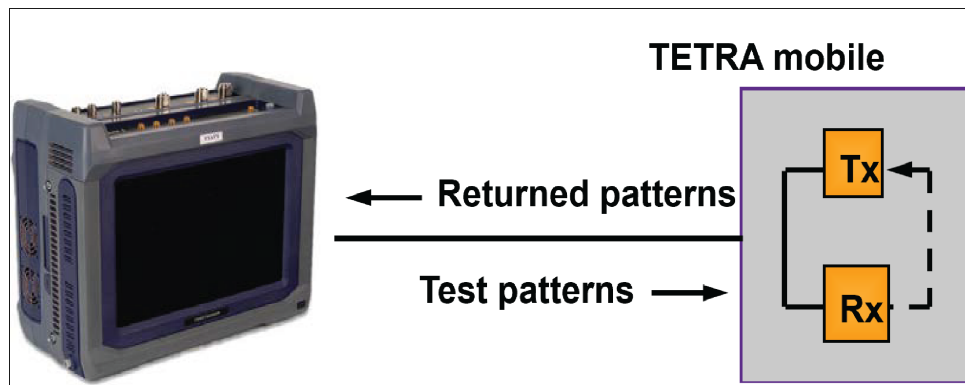
Figure 3-11 TETRA Loopback BER Test Setup Diagram
