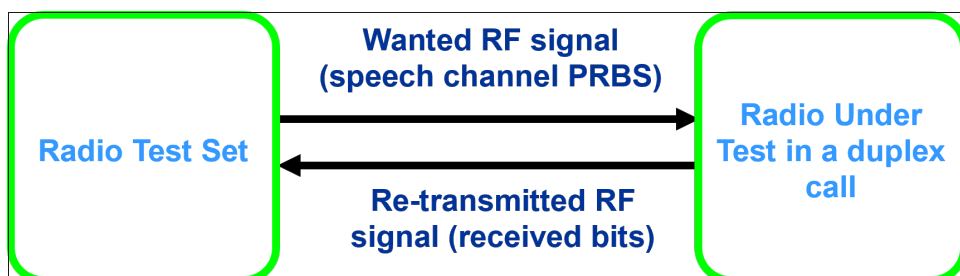
Figure 3-10 TETRA TT Mode Duplex Call Loopback Configuration
