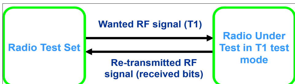
Figure 3-9 TETRA T1 Test Mode Loopback Configuration
