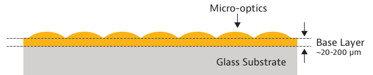
Polymer-on-glass Diffuser
