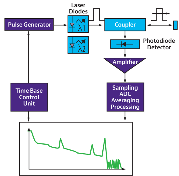
OTDR block diagram
