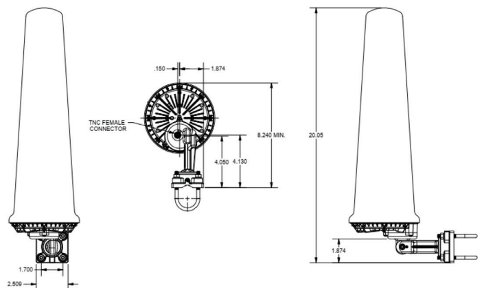
SecureTime altGNSS GEO-L Helical Antenna Dimensions
