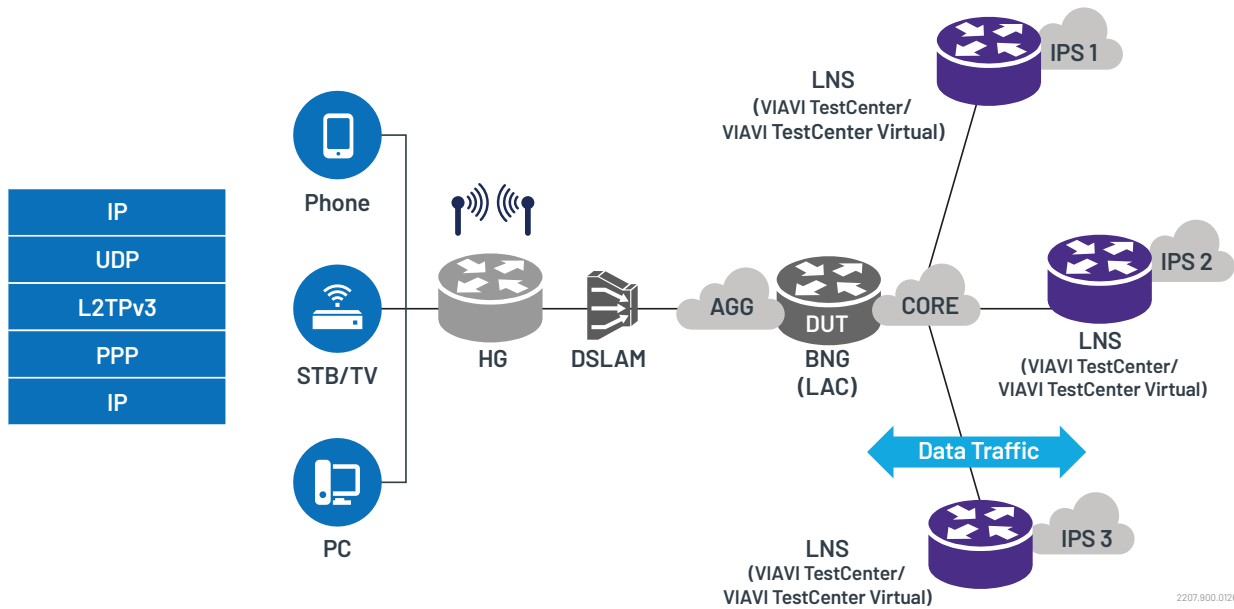
Broadband Access Testing Topology
