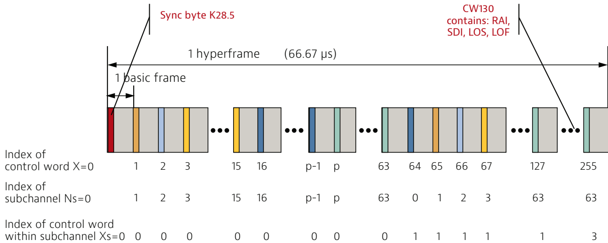
Figure 5. CPRI frame structure
