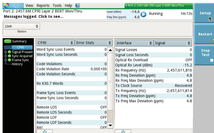
Figure 7. CPRI test results
