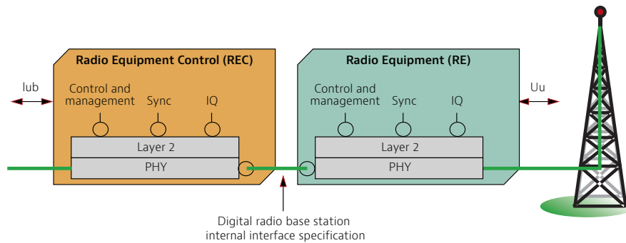
Figure 2. A CPRI interface
