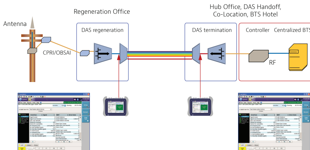
Figure 8. Testing xWDM-based fronthaul networks
