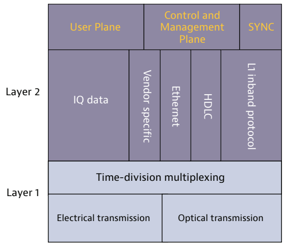
Figure 3. CPRI protocol layers
