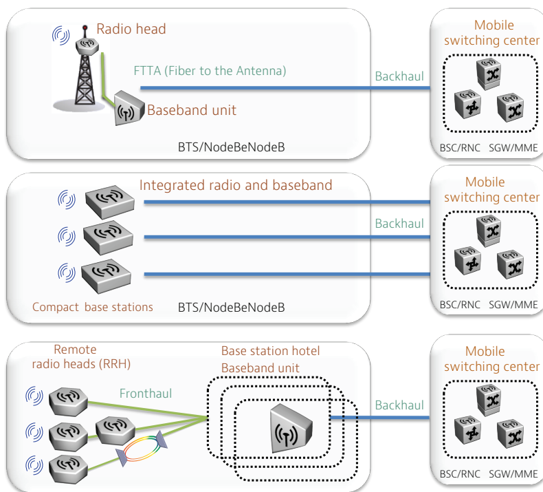
Figure 1. Evolution of cellular networks
