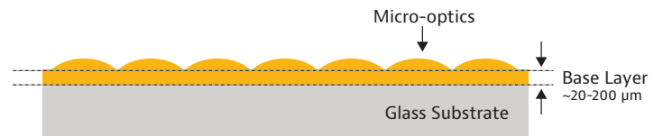
Polymer-on-glass Diffuser
