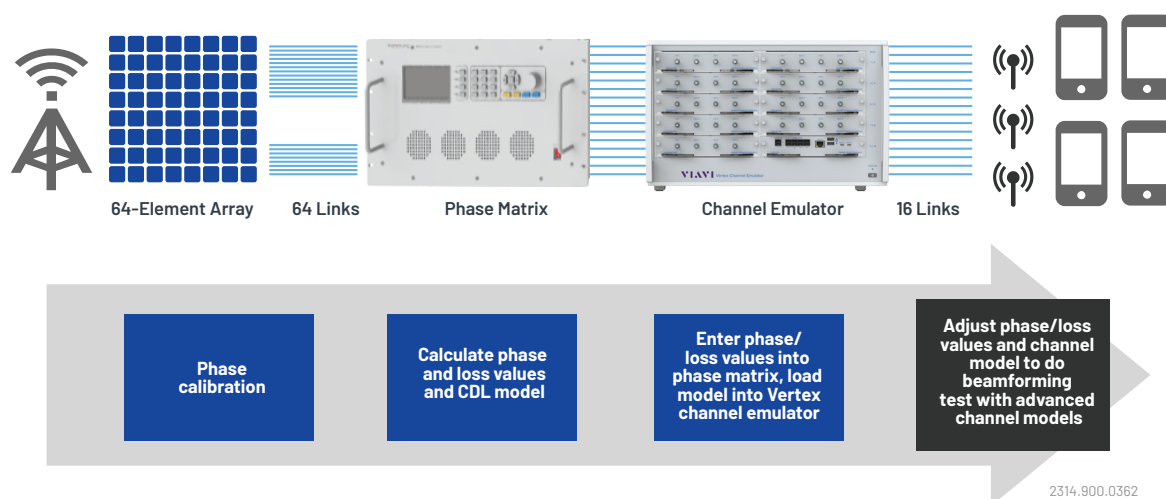
Figure 4. Advanced beamforming test with phase matrix and Vertex channel emulator
