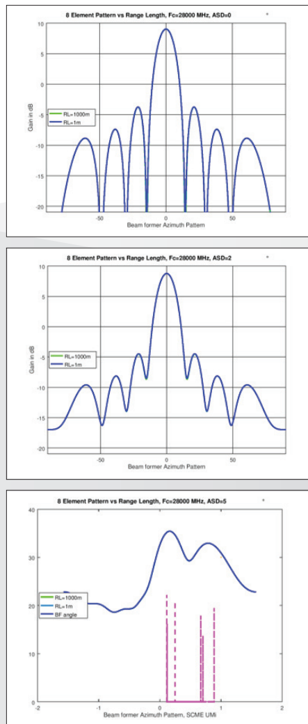
Figure 2. Examples of beamforming under different propagation conditions
