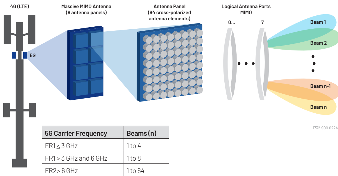
5G Massive MIMO and Beamforming
