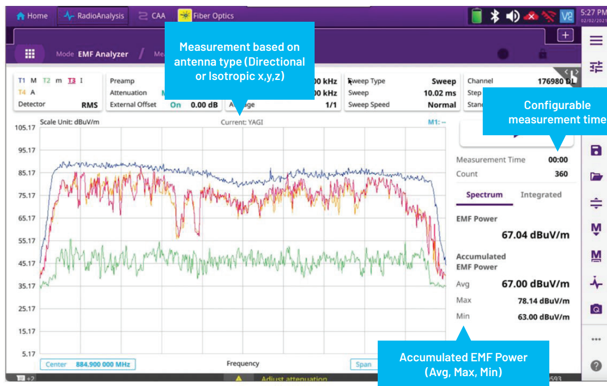
OneAdvisor 800 Wireless EMF Spectrum Analysis (frequency selective mode)
