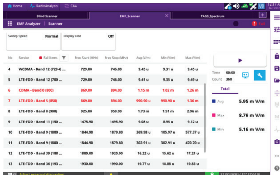
OneAdvisor 800 Wireless EMF Scanner (frequency selective mode)
