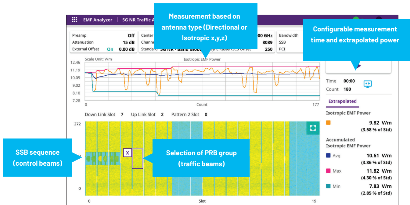
OneAdvisor 800 Wireless 5G EMF Traffic Analysis (code selective mode)
