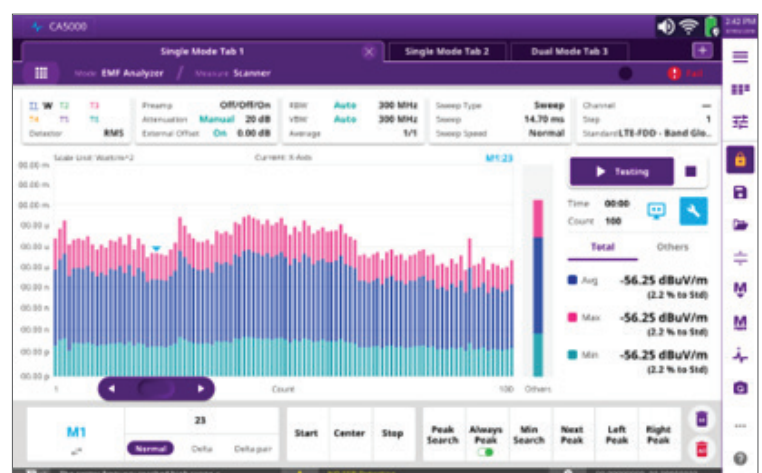
OneAdvisor 800 Wireless EMF Scanner (frequency selective mode)
