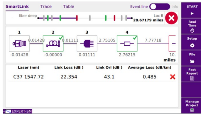
xWDM Link Mapping
