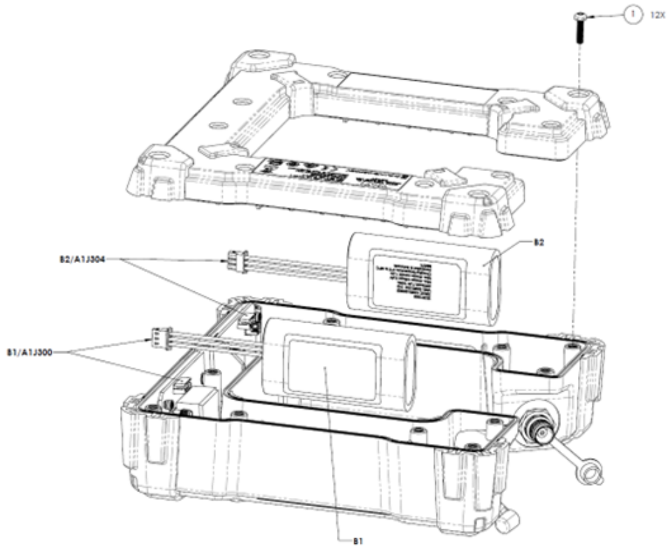
Figure 7-1 Base Cover Removal
