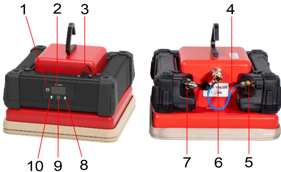
Figure 1-4 OSPREY Controls and Connectors
