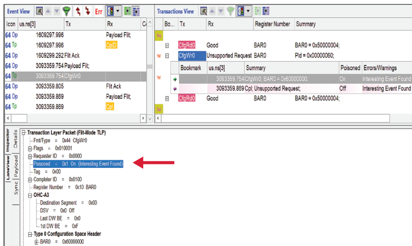
Observed result – UR completion, BAR0 unchanged, confirming EP bit detection
