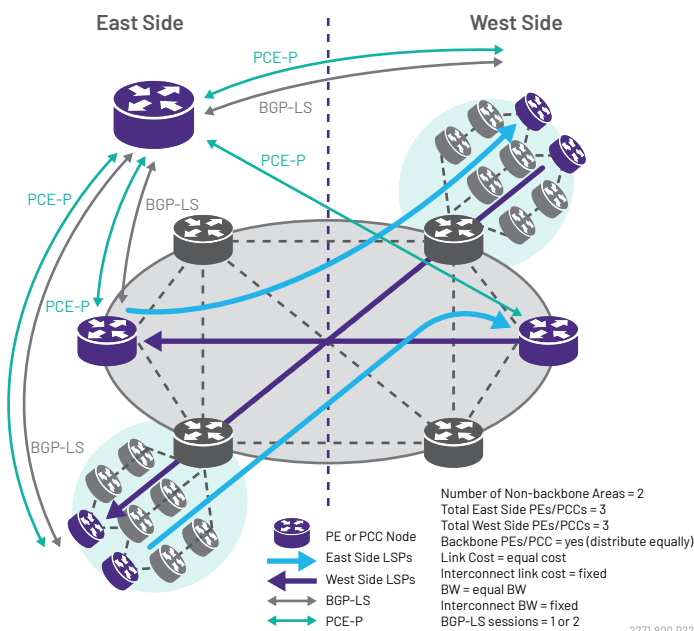
Figure 1: Multi-area BGP-LS Test Topology
