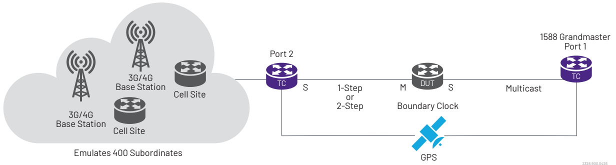
1588 Boundary Clock Testing
