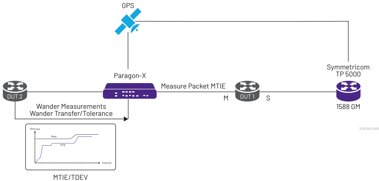
1588 PDV and G.8261 Testing
