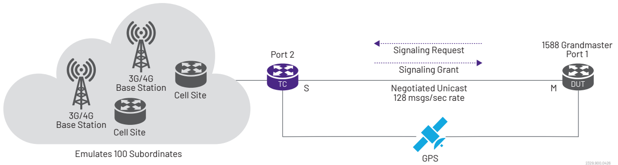
1588 Telecom Profile Testing
