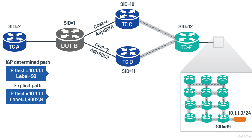
Segment Routing Test Topology
