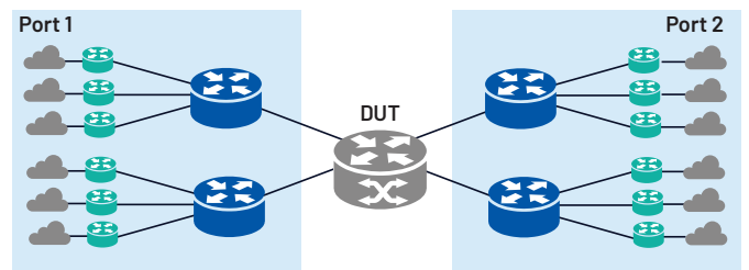
Unicast Router Test Topology
