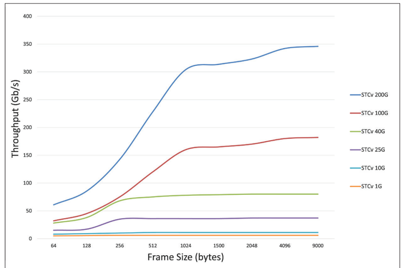
Figure 2. VIAVI TestCenter Virtual Performance
