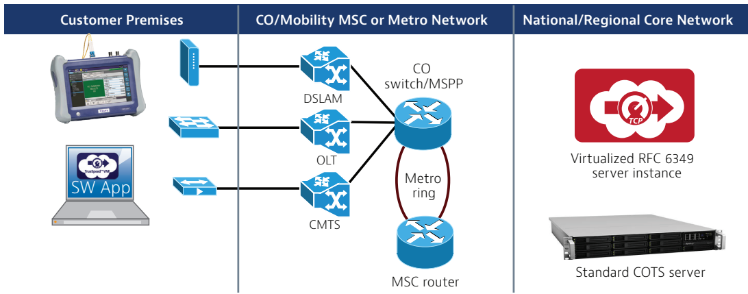
TrueSpeed VNF — architecture, software, and hardware elements
