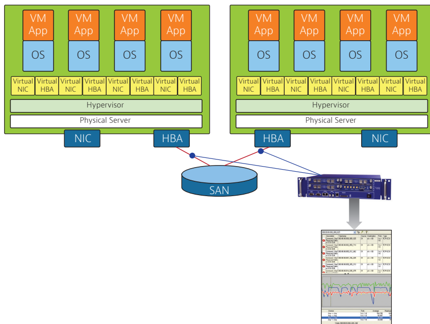
Figure 5. VM SAN with Xgig
