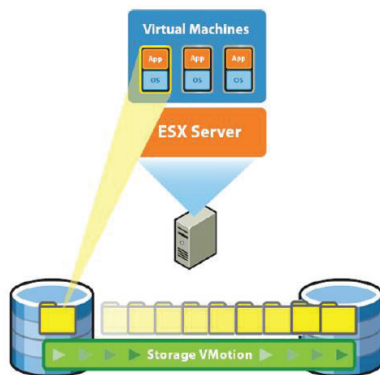
Figure 2. VMWare
