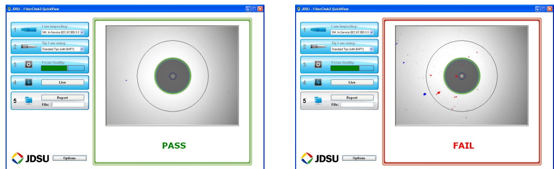
Figure 2: Example of the Proven Inspection and Analysis Software Program FiberChek2 from JDSU
