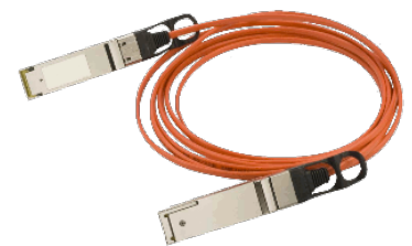
Figure 2. AOC Cable
