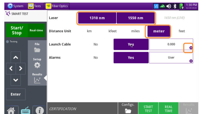
Figure 5: SMART TEST Setup
