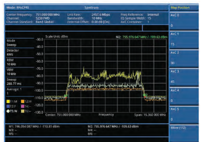
RFoCPRI — Spectrum
