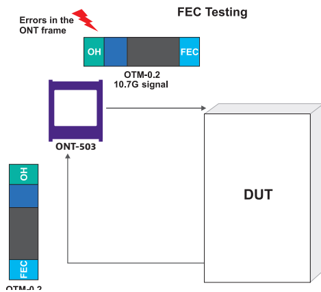
Figure 22: FEC test setup
