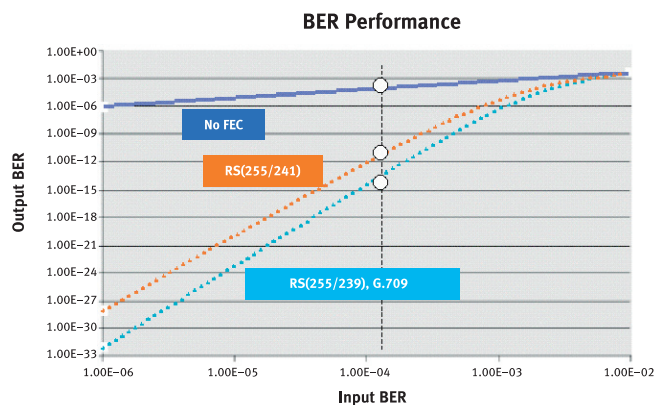
Figure 18: Effect of using FEC with various algorithms
