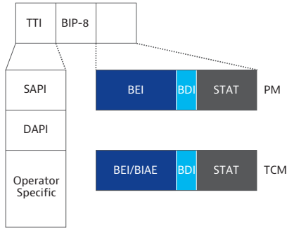
Figure 12: TCM and PM overhead structures
