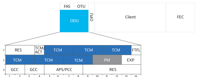
Figure 11: Overhead structure of ODU
