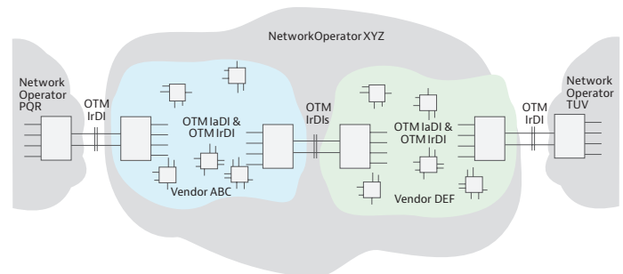
Figure 3: ITU-T G.872 definition of network interfaces
