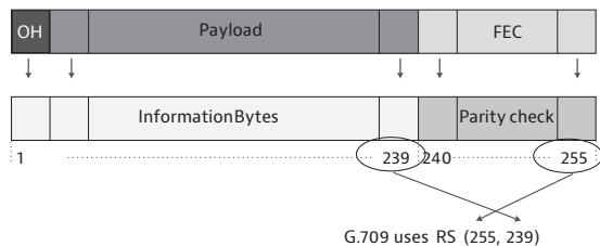
Figure 17: Forming of parity check
