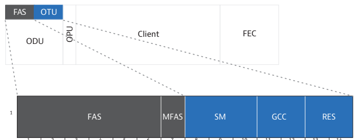
Figure 7: Frame alignment and OTU OH structure
