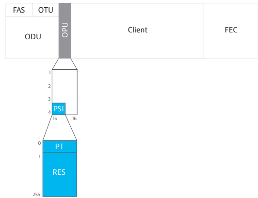
Figure 10: Overhead of OPU
