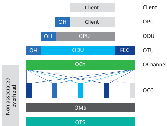
Figure 1: Basic OTN transport structure
