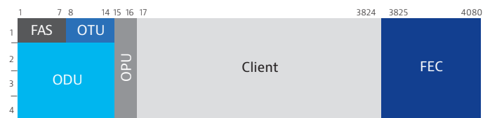
Figure 6: Optical channel structure consisting of OH bytes, client, and FEC
