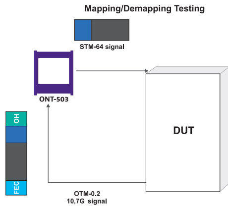
Figure 21: Conducting mapping and demapping tests
