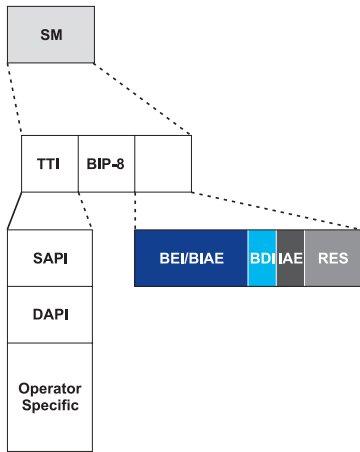
Figure 8: Section monitoring OH
