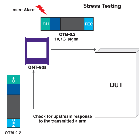
Figure 20: Setup for stimulus testing
