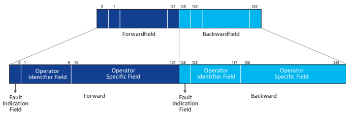
Figure 14: Structure of the FTFL field with its corresponding substructure
