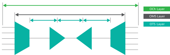
Figure 4: OTN layer structure; as with SONET/SDH, the OTN has a layered structure design
