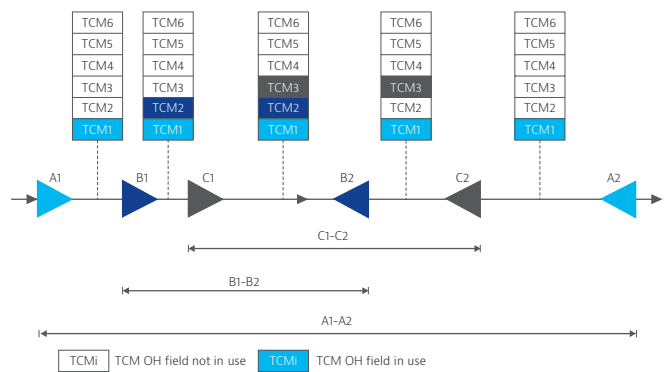
Figure 13: Possible TCM structure in an OTN
