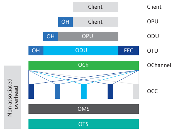
Figure 5: Basic OTN transport structure
