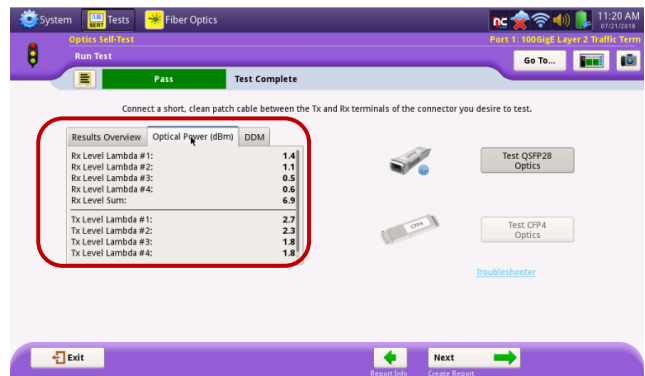
Figure 9: Optical Power (dBm) Results (100GBASE-LR4 optics)
