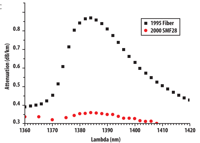
Fiber Attenuation Comparison
