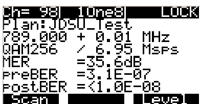
The MSQ-800 performs QAM testing on QAM-64/256 providing results for MER and Pre/Post-BER measurements.
