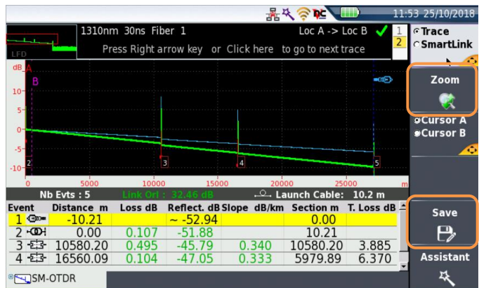
Figure 11: Trace View
