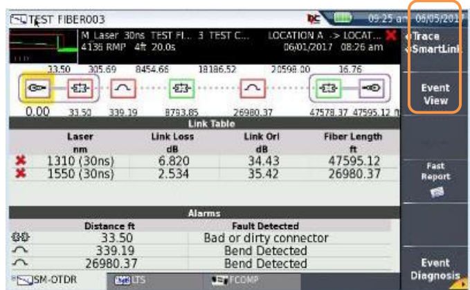
Figure 10: SmartLink View
