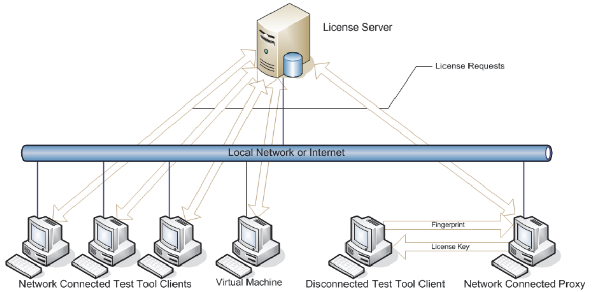
Figure 1 Medusa Licensing Model
