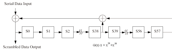
Figure 2. The scrambling process for LAN PHY patterns 1 and 2
