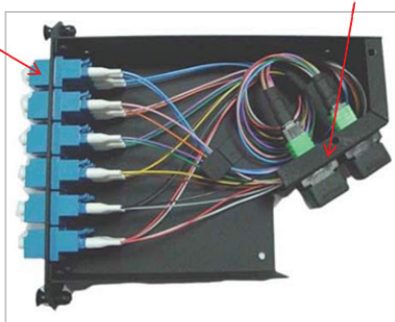
Back plate
