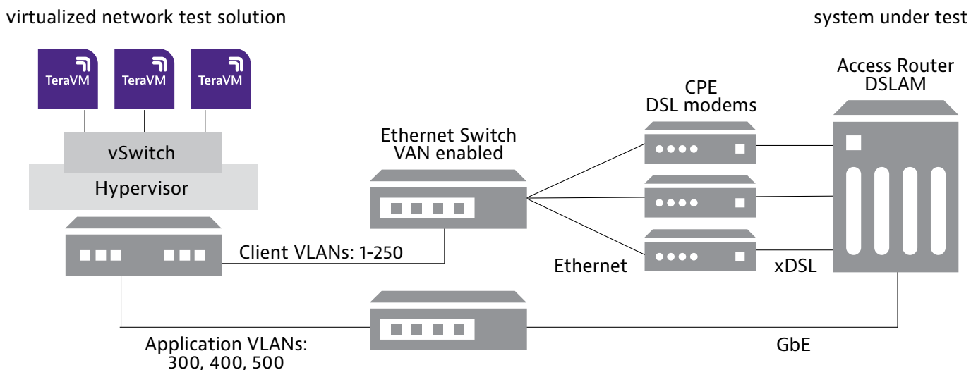
Figure 1: TeraVM's emulated endpoints with unique VLAN tags.
