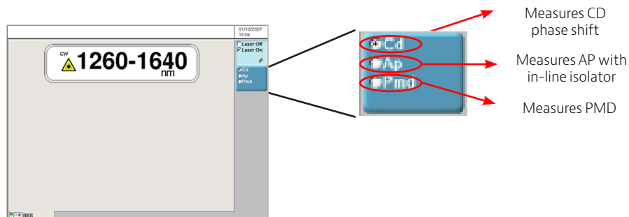
Figure 1. Source configuration
