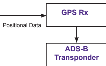
GPS Simulator
