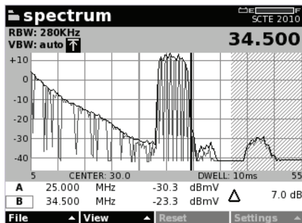
Figure 4. Spectrum with Long Dwell Time
