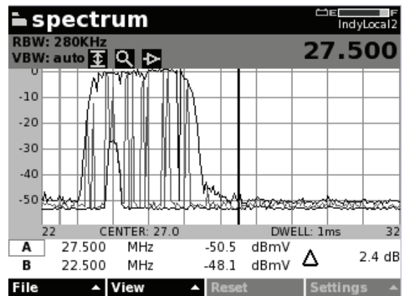
Figure 2. Spectrum with Minimum Hold Trace
