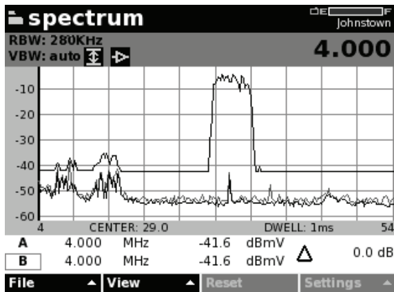
Figure 1. Spectrum with Pre-Amp
