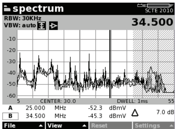
Figure 3. Spectrum with LPF Enabled
